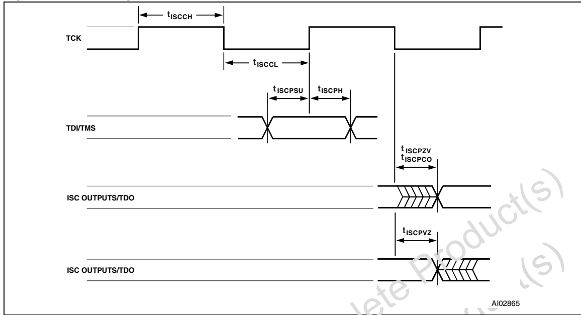
Figure 52. ISC Timing
